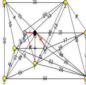
FIG. 6 – The example for algorithm BIP-step2 : 10→6
