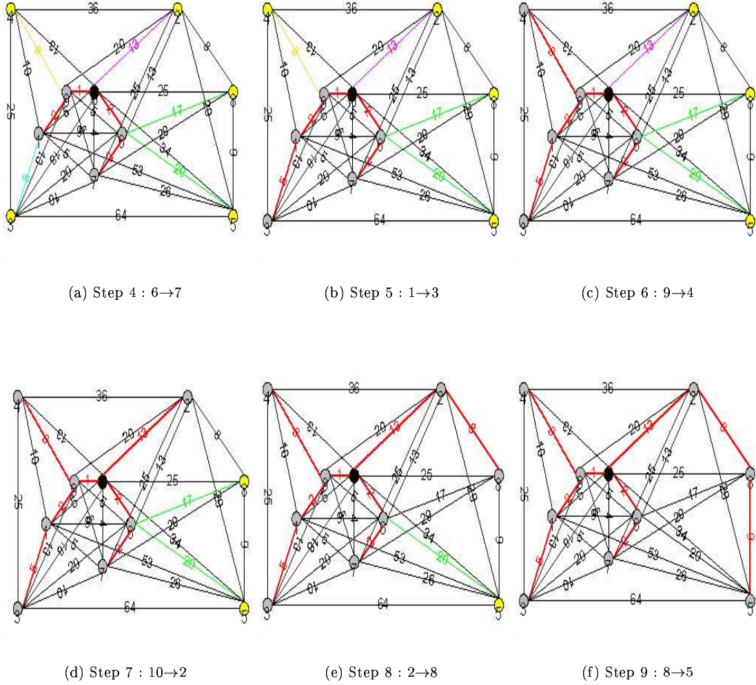
FIG. 29 – The example for algorithm MRN-MST step4-9
