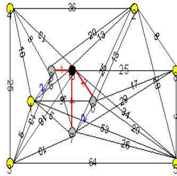
FIG. 34 – The network example of MRN-BIP step3 : 10→7
