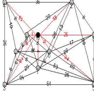
FIG. 31 – The broadcast tree obtained by MRN-EWMA- e_{MRN-EWMA} = 34
