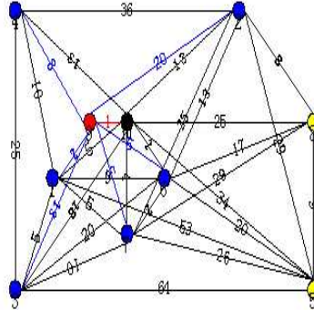
FIG. 11 – The example for algorithm MBT step1
