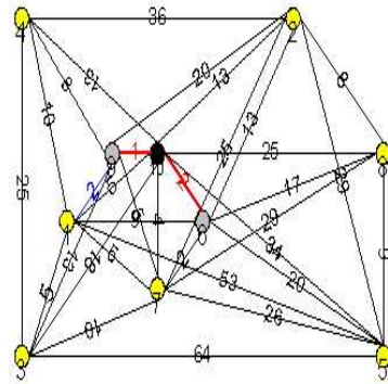
FIG. 33 – The network example of MRN-BIP step2 : 10→6
