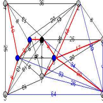
FIG. 9 – Final tree obtained by algorithm BIP- e_{BIP}=34
