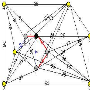
FIG. 7 – The example for algorithm BIP-step3 : 6→7
