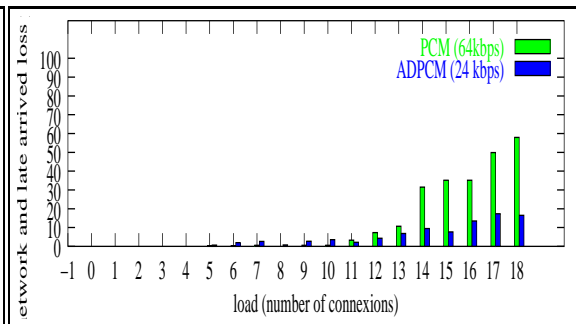
FIG. 13 – Averaged network and late arrivals loss percentage as a function of load traffic (OLSR)
