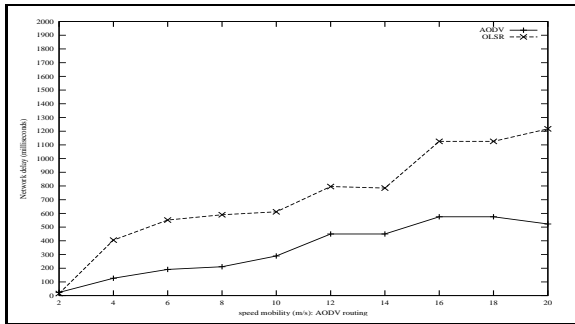
FIG. 14 – Averaged end-to-end delay as a function of mobility speed: AODV and OLSR
