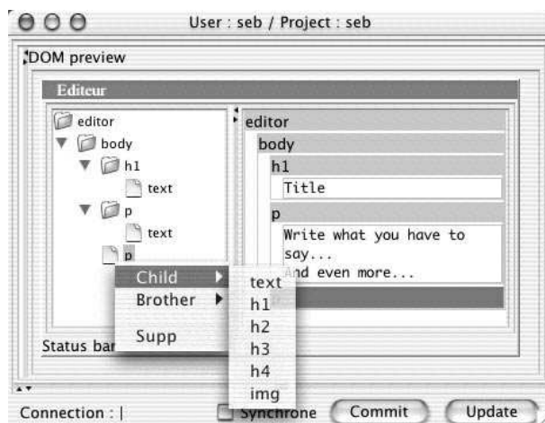
Figure 2. SAMS-XML editor
