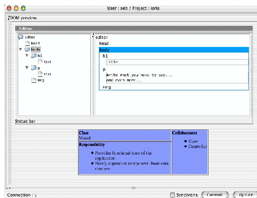
Figure 3. SAMS-XML environment
