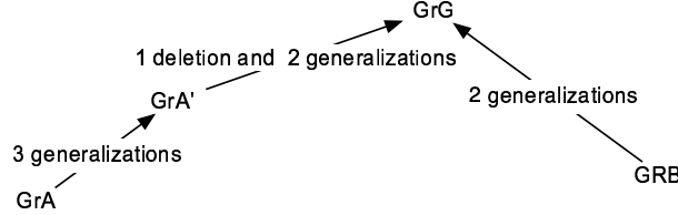
Figure 6: The similarity-path between graphs GrA and GrB .
