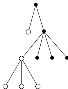
Figure 25: Tree with visible subtrees; TCs is the default filled disk. (after page 39 of [16])
