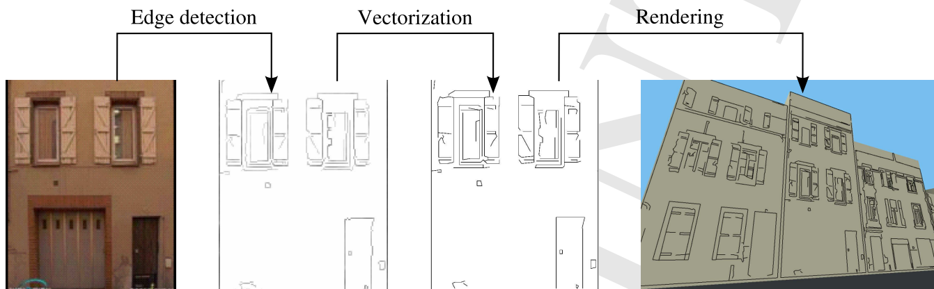
Figure 1: Production pipeline of stroke-based buildings. The edges of facade images are extracted and vectorized. This vector data is used instead of textures to represent the facade in the final 3D model.
