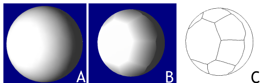
Figure 1: A: original bitmap; B: vector approximation (8 primitives with linear gradients); C: the primitives.
