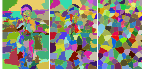
Figure 3: Influence of the parameter \lambda , weighting the cells compactness criterion. From left to right: \lambda = 0 uses the fitting term alone; \lambda = 0.75 constructs compact cells aligned with the features; \lambda = 1 ignores the fitting term and constructs a Voronoi tessellation.
