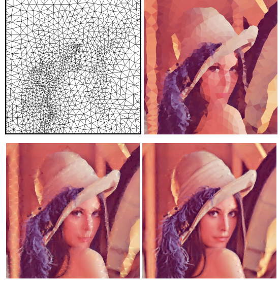
Figure 6: Trixels with the attached pre-integrated higher-order representation of degree 0, 1 and 2 (2000 trixels).
