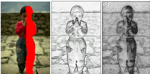
Figure 5: Constructing the intermediate “trixel” data structure. User-defined importance map (right part of the character), saliency map and resulting trixels, adapted to both maps.
