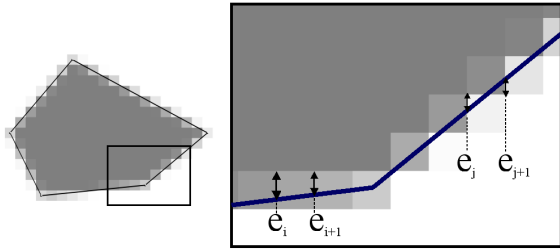
Figure 12: Using Bresenham's algorithm to compute exact integrals over images.
