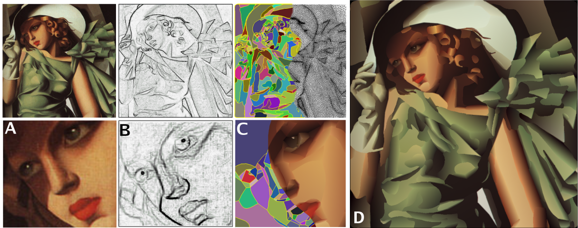
Figure 2: The principal steps of Ardeco to convert a bitmap image into vector primitives. A: original image; B: saliency estimation; C: saliency-adapted triangulation (trixels) and partition into regions; D: final result (240 cubic splines filled with gradients)
