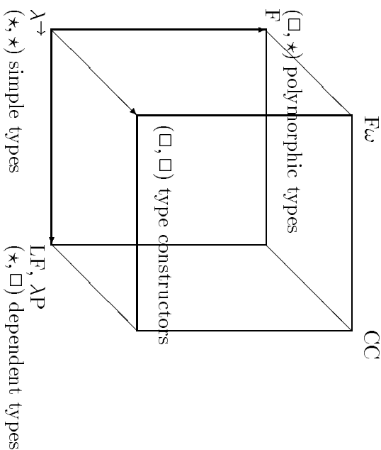
Figure 1.2: Barendregt's Cube
