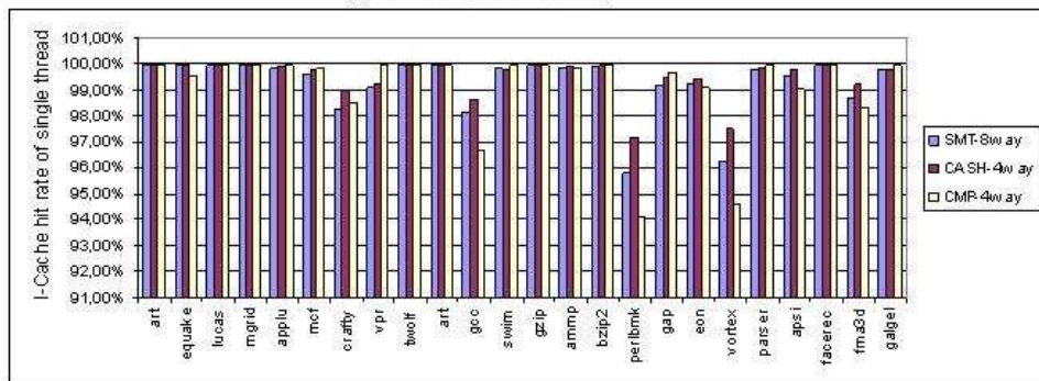
Figure 11: I-Cache hit rate in three architectures with different issue widths.
