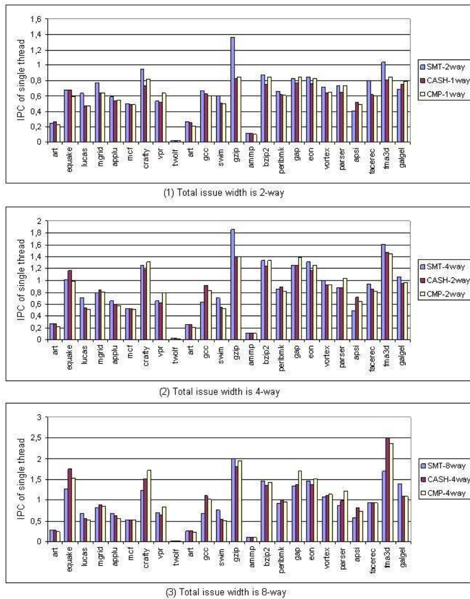
Figure 9: Single thread performance in three architectures with different issue widths.
