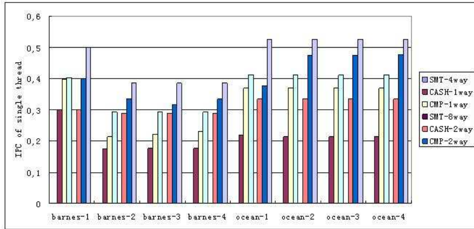
Figure 25: Single thread performance of parallel workloads in 4-thread mode with different issue widths.
