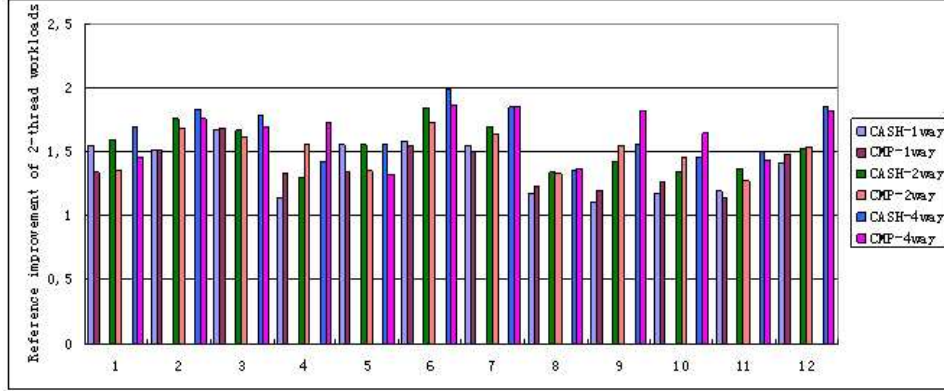
Figure 8: Reference improvement of 2-thread workloads on CASH and CMP.
