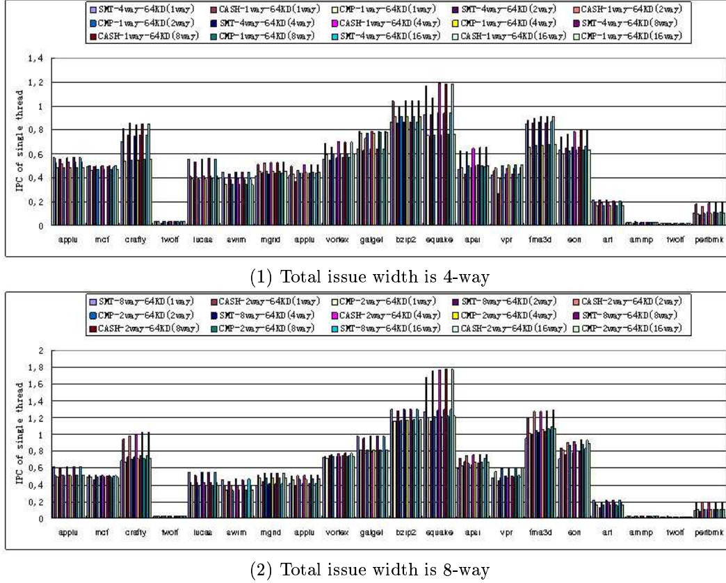
Figure 40: Performance of single thread in 4-thread workloads with different D-Cache associativity.
