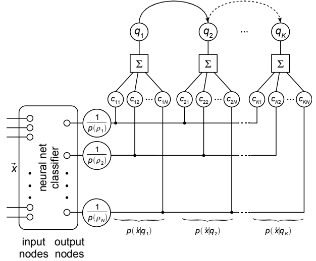
Figure 1. Combination of a neural net and semi-continuous HMM for the tied posterior approach.
