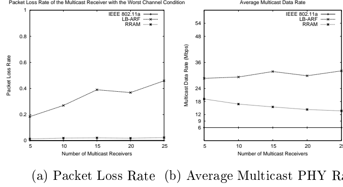
Figure 8: Packet loss rate and multicast PHY rate comparison.
