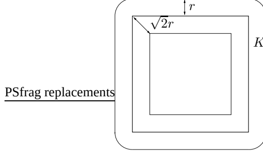
Figure 5: The boundary of the r -offset of a square K in the plane is at Hausdorff distance \sqrt{2}r of K . For \mu = \frac{\sqrt{2}}{2} , r_\mu(K) > 0 and this example shows the tightness of the bound in theorem 3.2
