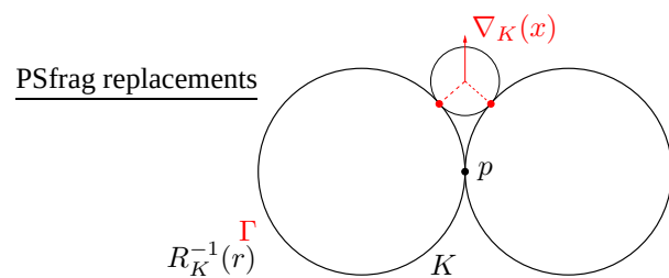
Figure 8: The union of two tangent discs in the plane has a positive wfs and zero \mu -reach for any \mu \in (0, 1) : if p is the intersection point of the two discs, then \nabla_K(x) tends to 0 as x \in K^c tends to p
