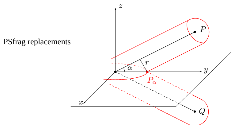
Figure 9: Tightness of the bound
