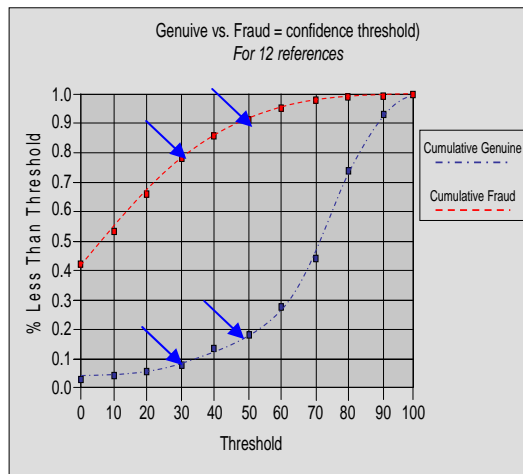
Figure 6: Cumulative Distributions for Genuine and Fraud Signatures
