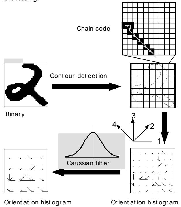
Figure 4 Features derived from contour chain code
