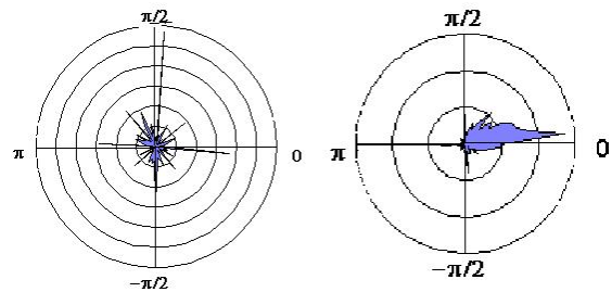
Figure 12. Directions of (a) starting and (b) ending
