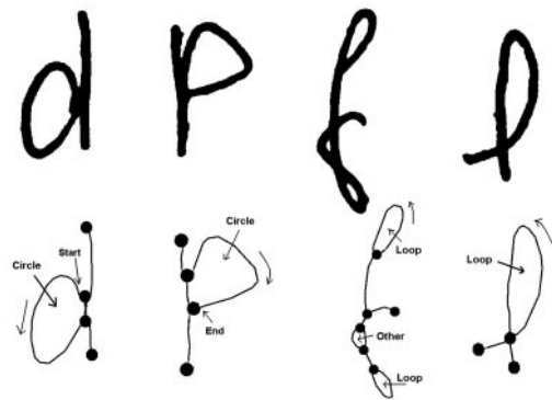
Figure 6. Labelling and crossing cycles
