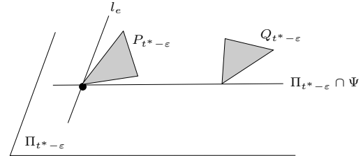
Figure 10: The set u of supports of line \Pi_{t^* - \epsilon} \cap \Psi is a maximal (P_t, Q_t) -tuple for some but not all t in any open neighborhood of t^* . There is a F-critical event (t^*, m) (where m = \Pi_{t^*} \cap \Psi ) such that u is contained in the set of supports of m because (i) m lies in plane \Psi \neq \Pi_{t^*} containing a face of \mathbf{P} and (ii) m is tangent to \mathbf{P} \cap \Psi at some point not on l_e . Note that there is no V-critical event (t^*, v) such that u contains v or an edge with endpoint v , and there is no line \ell \in \Pi_{t^*} such that (i) \ell lies in a plane \Upsilon \neq \Pi_{t^*} containing a face of \mathbf{P} and (ii) \ell is tangent to \mathbf{Q} \cap \Upsilon at some point not on l_e ; indeed \ell is necessarily equal to m , if \Upsilon = \Psi then \ell is not tangent to \mathbf{Q} \cap \Upsilon and we can consider that the plane, distinct from \Psi , that contains \ell and a face of \mathbf{P} is equal to \Pi_{t^*} .
