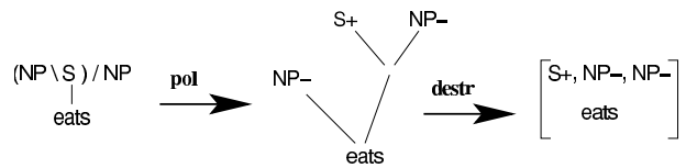
Figure 3: Syntactic structures associated with the transitive verb eats in LG, \text{LG}_{pol} , (\text{LG}_{pol})_{destr}
