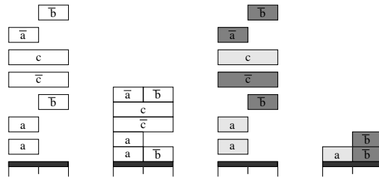
Figure 1: A heap in \mathbb{M}(\tilde{\Sigma}, \tilde{I}) (left) and a colored heap in \mathbb{F}(\Sigma, I) (right).
