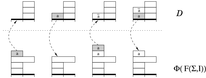
Figure 3: The involution \psi . From left to right, the cases are 1,2,4, and 3.
