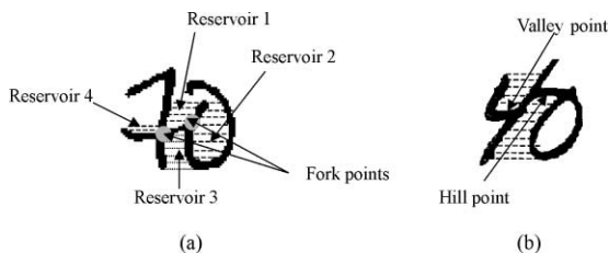
Fig. 4. Example of (a) fork points, (b) hill and valley points obtained by reservoir.
