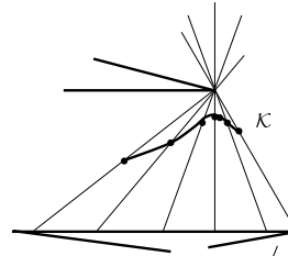
FIG. 5.6. Relevant 2-contact tracing of type (wall-endpoint) 2 , i.e., arc of ellipse.
