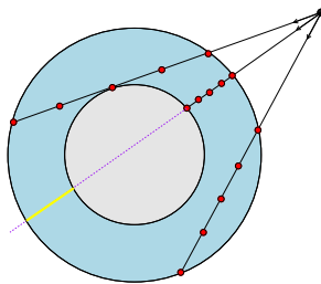
Figure 7: This figure illustrates how rays from a fixed point of view are marched adaptively depending on their length and on the number of samples that has been predefined (for illustration purpose, we chose 5 samples per ray). Notice the ray traversing two times the tokamak, only the nearest integration is taken into account, the yellow sub part being ignored.
