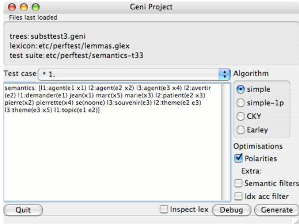
Figure 1. The main user interface
