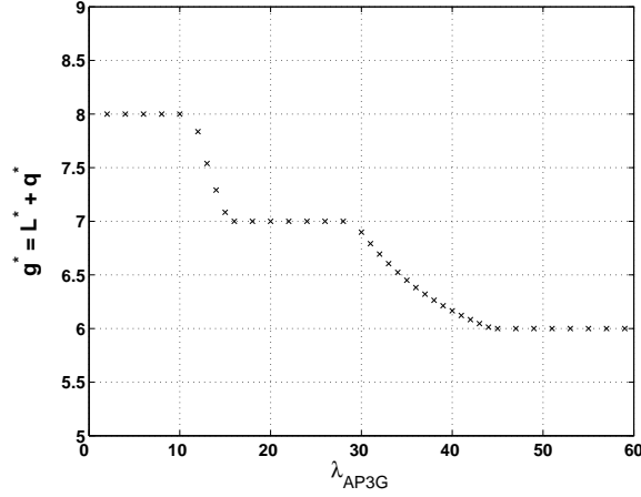
Figure 11: g^* \text{ v/s } \lambda_{AP3G} for \lambda_{AP} = 3 , M_{AP} = 10 and \tau = 2.5
