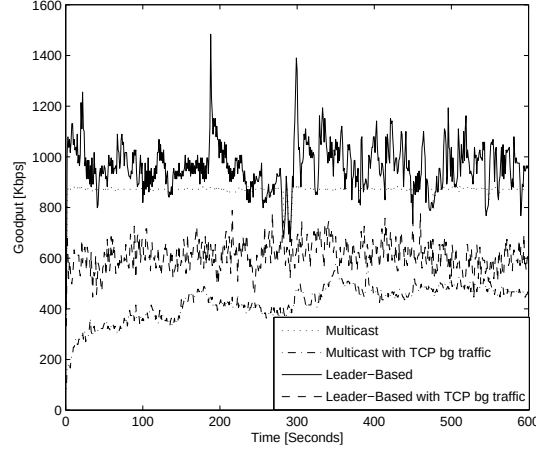
Figure 12: Video goodput for legacy multicast and leader-based mechanisms
