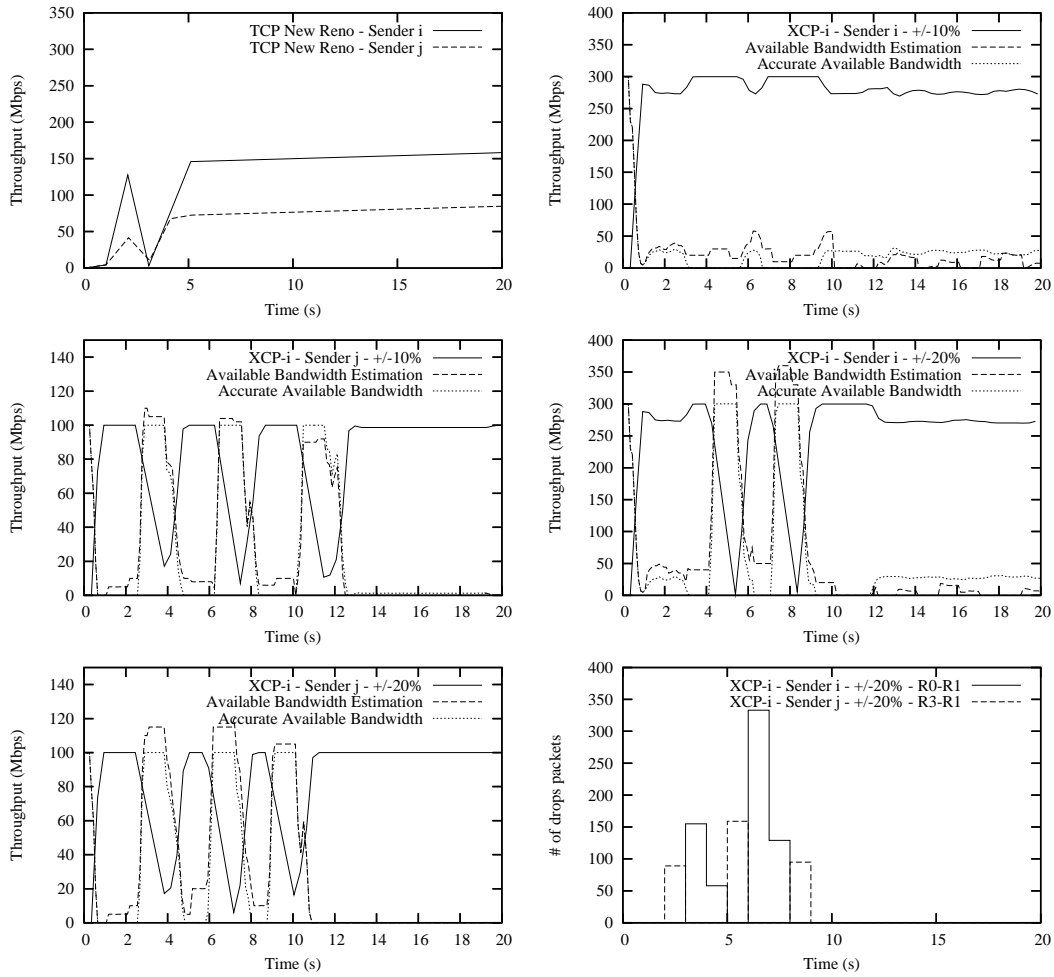
Figure 13: Top: throughput for TCP (left), XCP-i - Sender i - 10% (right). Middle: throughput for XCP-i - Sender j - 10% (left), XCP-i - Sender i - 20% (right). Bottom: throughput for XCP-i-Sender j-20%, packet losses XCP-i-20% (right).
