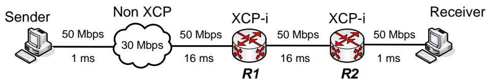
Figure 4: Asymmetric deployment: optimized receiver side
