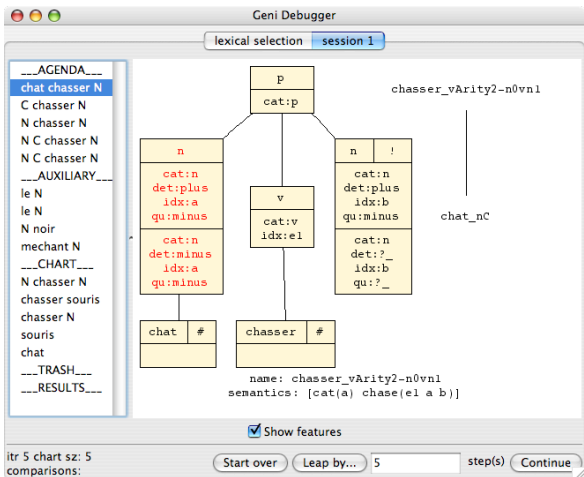
Figure 4: The GenI debugger
