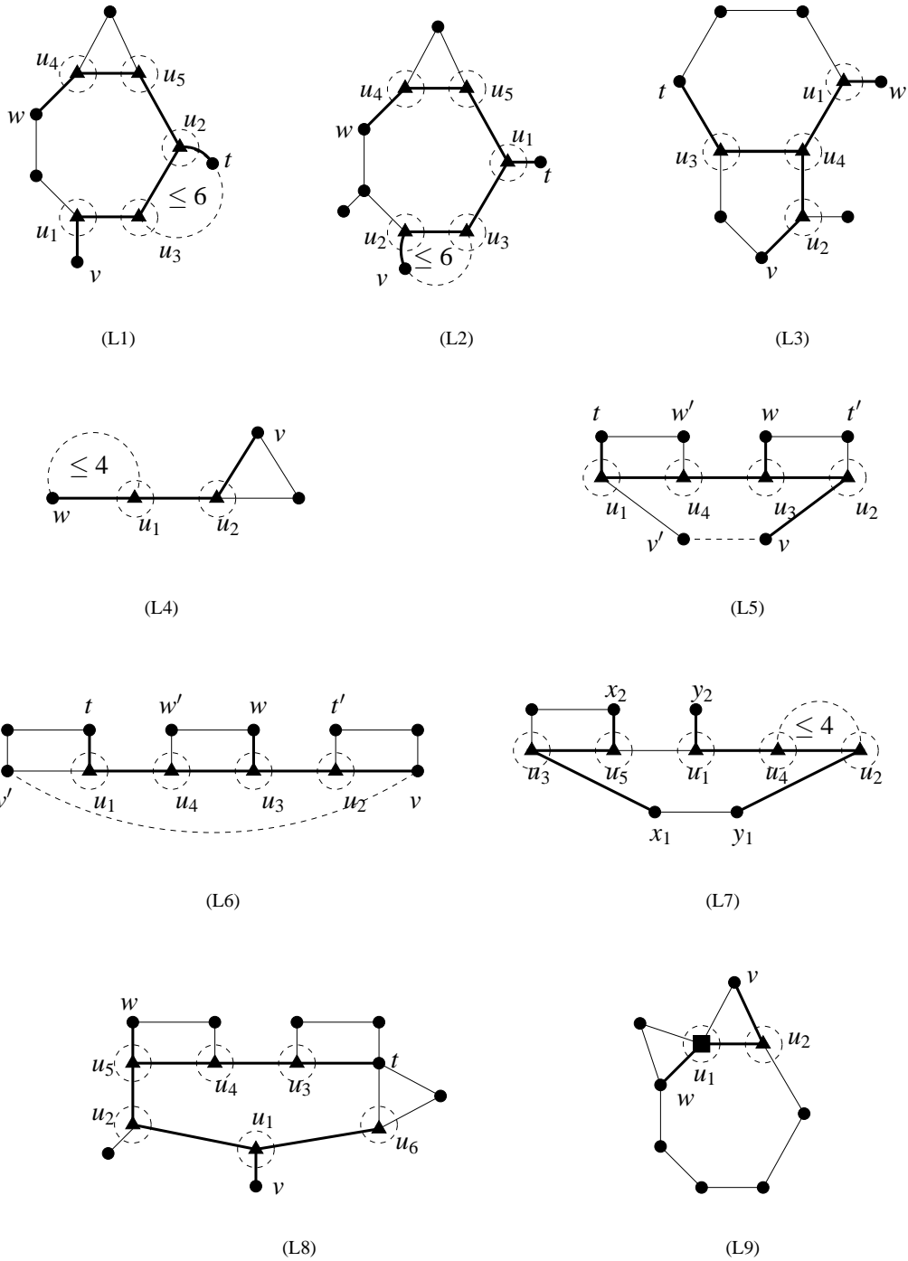
Figure 2: Reducible configurations (L1)–(L9).
