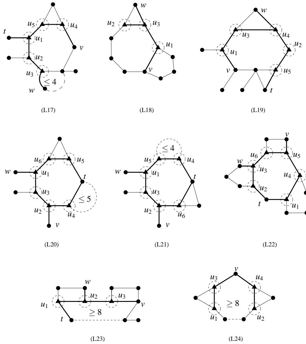
Figure 4: Reducible configurations (L17)–(L24).
