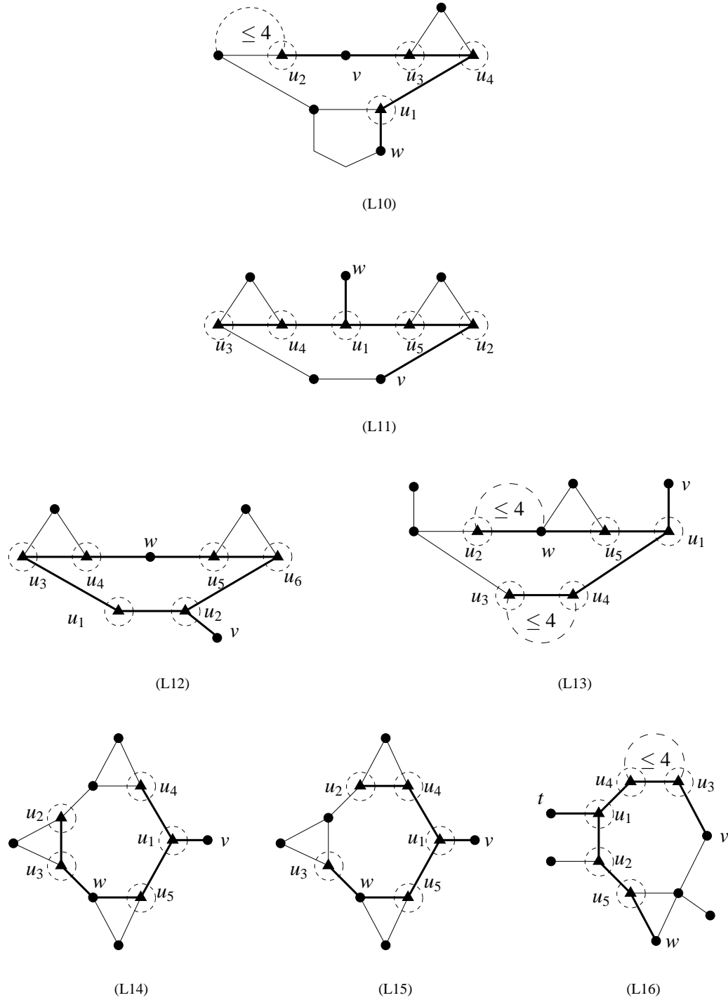
Figure 3: Reducible configurations (L10)–(L16).
