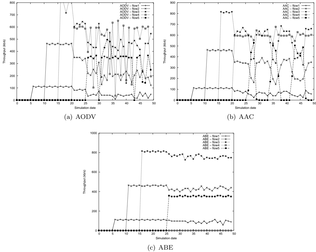
Figure 5: One-hop flows throughputs with AODV, AAC and ABE
