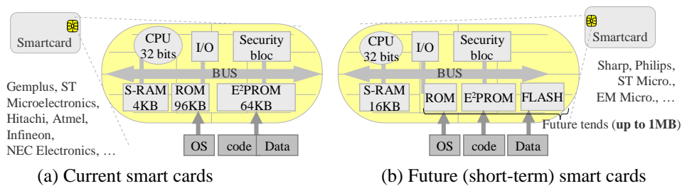
Figure 1. Typical smart cards architectures.
