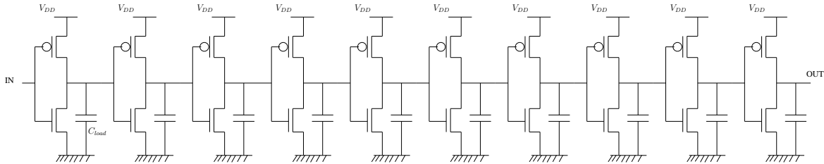
Figure 4.12: Inverter chain in CMOS
