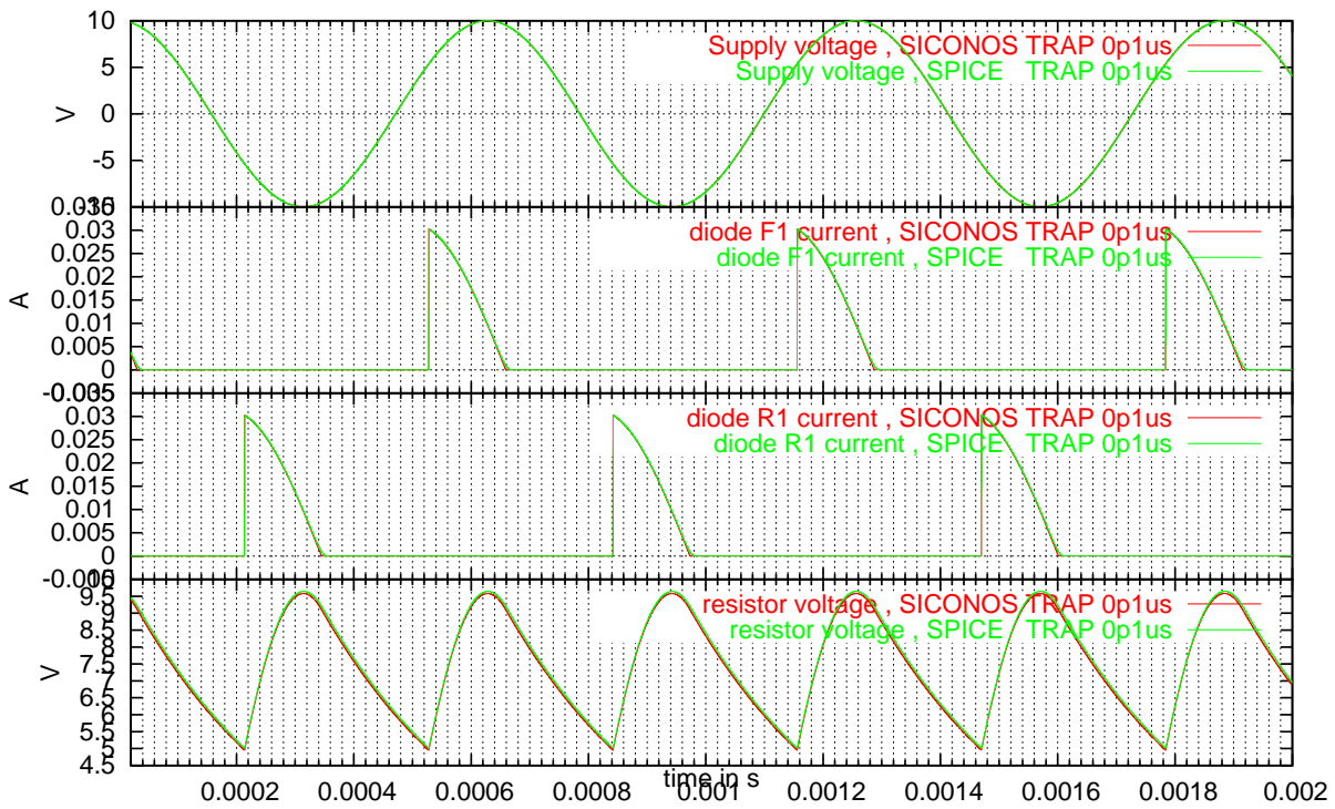
Figure 4.5: SPICE and SICONOS simulations of the diode bridge circuit, 0.1 \mu\text{s} time step
