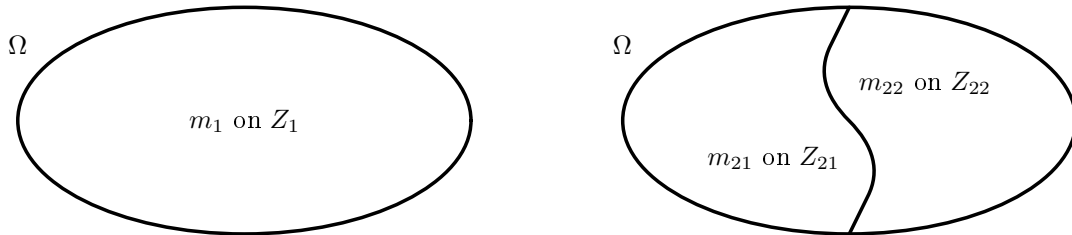
Figure 1: Refinement of a single-zone zonation represented in a two-dimensional space for simplicity. Left: one-zone parameterization \mathcal{P}_1 with \bar{\Omega} = Z_1 (i.e. J_1 = \{1\} ). Right: two-zone parameterization \mathcal{P}_2 with \bar{\Omega} = Z_{21} \cup Z_{22} (i.e. J_2 = \{21, 22\} ).
