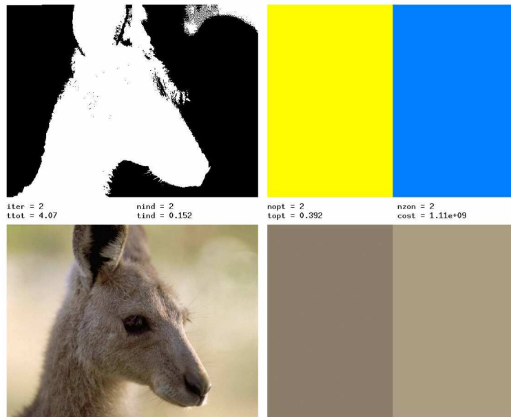
Figure 6: Dichotomy strategy, 2 zones. Bottom: data image d (left), segmented image p_2^{\text{opt}} (right). Top: pseudo-sign of the gradient g_2^{\text{opt}} (left), 2-zone zonation \mathcal{P}_2 (right). The refinement indicator for the first cutting was \mathcal{I}_1^{\text{dichotomy}} = 2.9 \cdot 10^6 .
