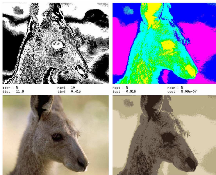
Figure 4: Best strategy, 5 zones. Bottom: data image d (left), segmented image p_5^{\text{opt}} (right). Top: pseudo-sign of the gradient g_5^{\text{opt}} (left), 5-zone zonation \mathcal{P}_5 (right). The refinement indicator for the fourth cutting was \mathcal{I}_4^{\text{best}} = 7.5 \cdot 10^5 .
