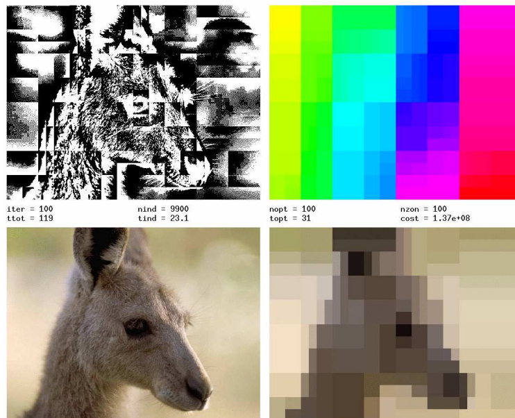
Figure 7: Dichotomy strategy, 100 zones. Bottom: data image d (left), segmented image p_{100}^{\text{opt}} (right). Top: pseudo-sign of the gradient g_{100}^{\text{opt}} (left), 100-zone zonation \mathcal{P}_{100} (right). The refinement indicator for the 99th cutting was \mathcal{I}_{99}^{\text{dichotomy}} = 2.8 \cdot 10^4 .
