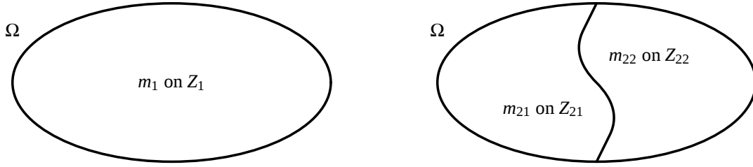
Figure 1: Refinement of a single zone zonation represented in a two-dimensional space for simplicity. Left: one-zone parameterization \mathcal{P}_1 with \overline{\Omega} = Z_{1,1} . Right: two-zone parameterization \mathcal{P}_2 with \overline{\Omega} = Z_{2,1} \cup Z_{2,2} .
