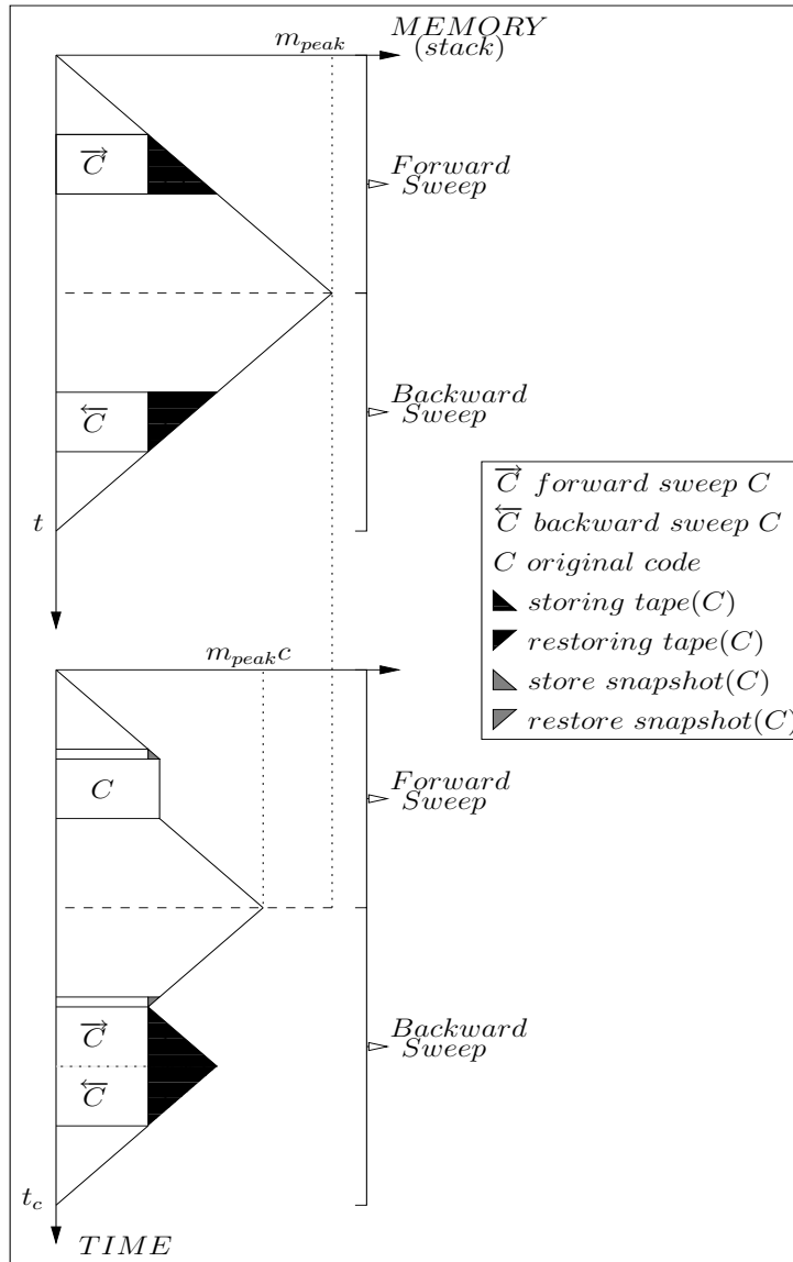
Figure 3: Checkpointing in Reverse Mode AD.
