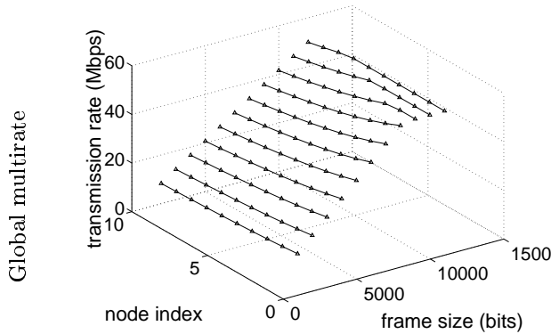
Figure 16: Using Equation 32, \zeta_i = 3
