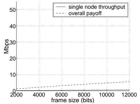
Figure 25: Using Equation 35, \zeta_i = e^6
