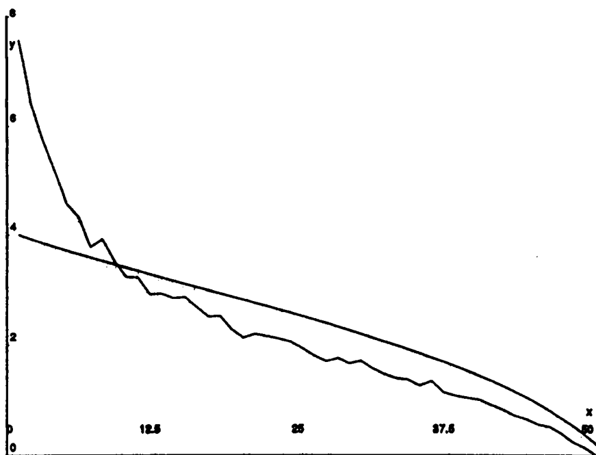
Figure 8: mean access delay versus position of a station. Input load \approx .8 , r = 5 with only N = 50
