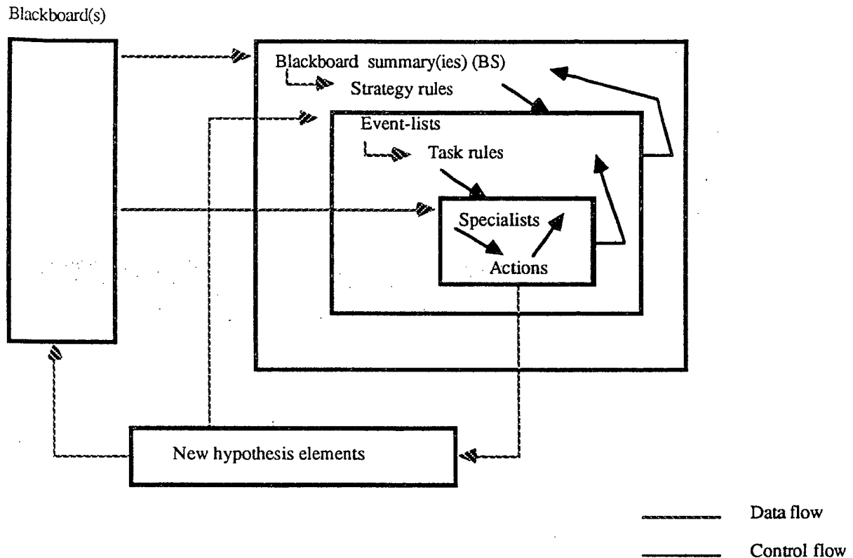
Figure 4 : ATOME's control structure (without the agendas).
