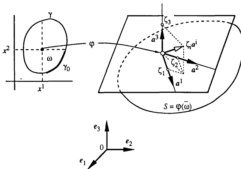
Figure 2.1 : In Koiter's model, the three unknowns are the covariant components \zeta_i : \bar{\omega} \rightarrow \mathcal{R} of the displacement \zeta_i \mathbf{a}^i of the points of the middle surface S = \varphi(\bar{\omega}) of the shell. The vectors \mathbf{a}^\alpha form the contravariant basis of the tangent plane, and \mathbf{a}^3 = \frac{\mathbf{a}^1 \times \mathbf{a}^2}{|\mathbf{a}^1 \times \mathbf{a}^2|} ; cf. Figure 1.1.
