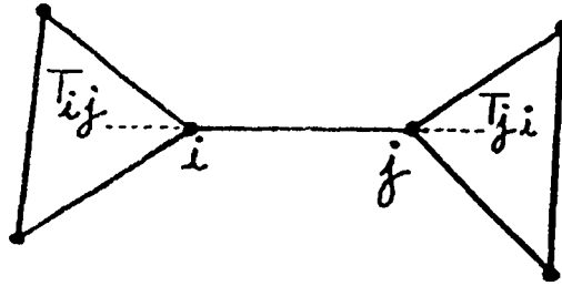
FIGURE 3 Upwind triangles for a given side ij
