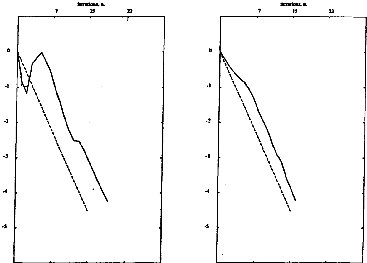
Figure 12: Convergence history of the implicit MG method based on \frac{1}{2} -upwind Osher's splitting explicitly, 1st-order Steger-Warming splitting implicitly, and 5-level multigrid for the implicit solution
