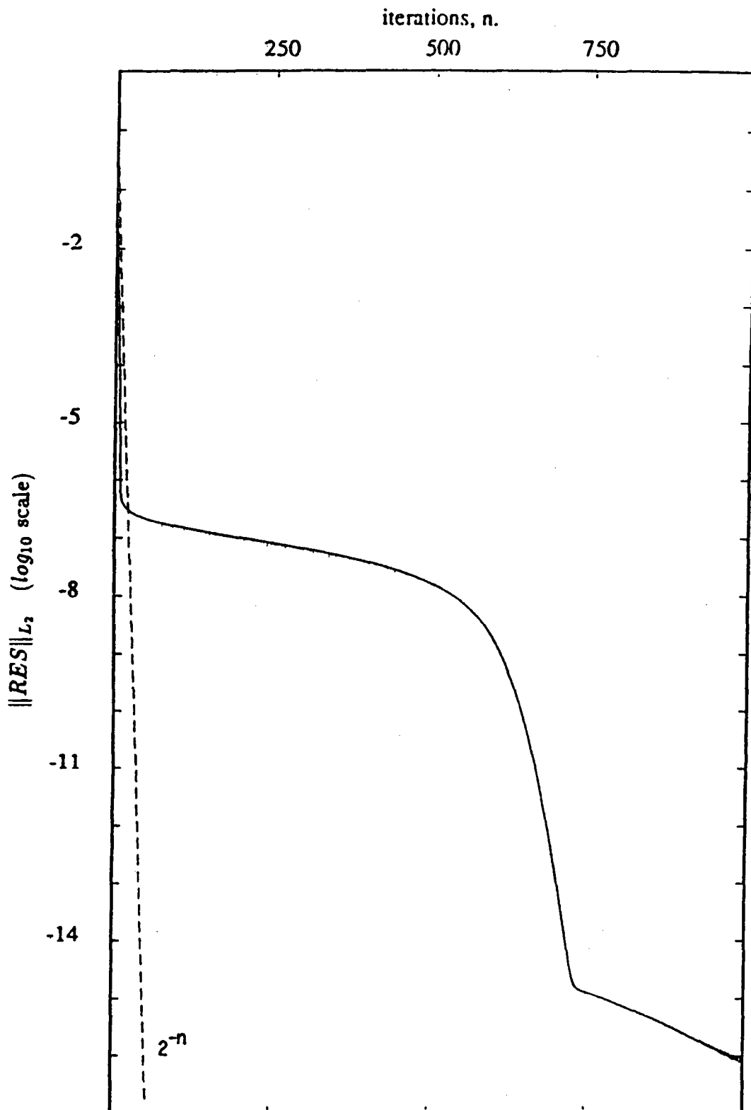
Figure 2 (c) : (c) central differencing scheme explicitly ( \beta = 0 )
