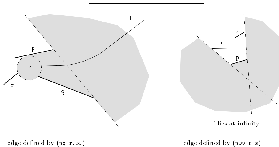
Figure 1.5 : Infinite edges
