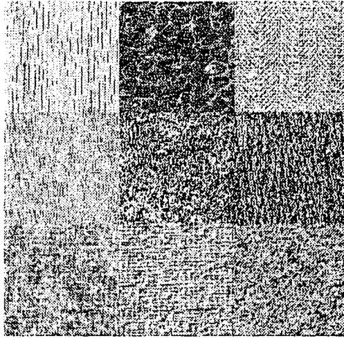
Figure 11: Brodatz textures
