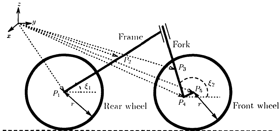
Figure 2. Bicycle model
