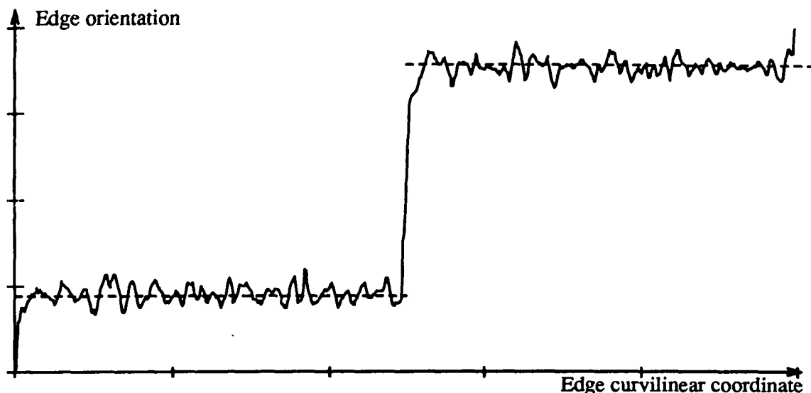
Figure 10: Computation of the orientation along two sides of a square in the presence of noise
