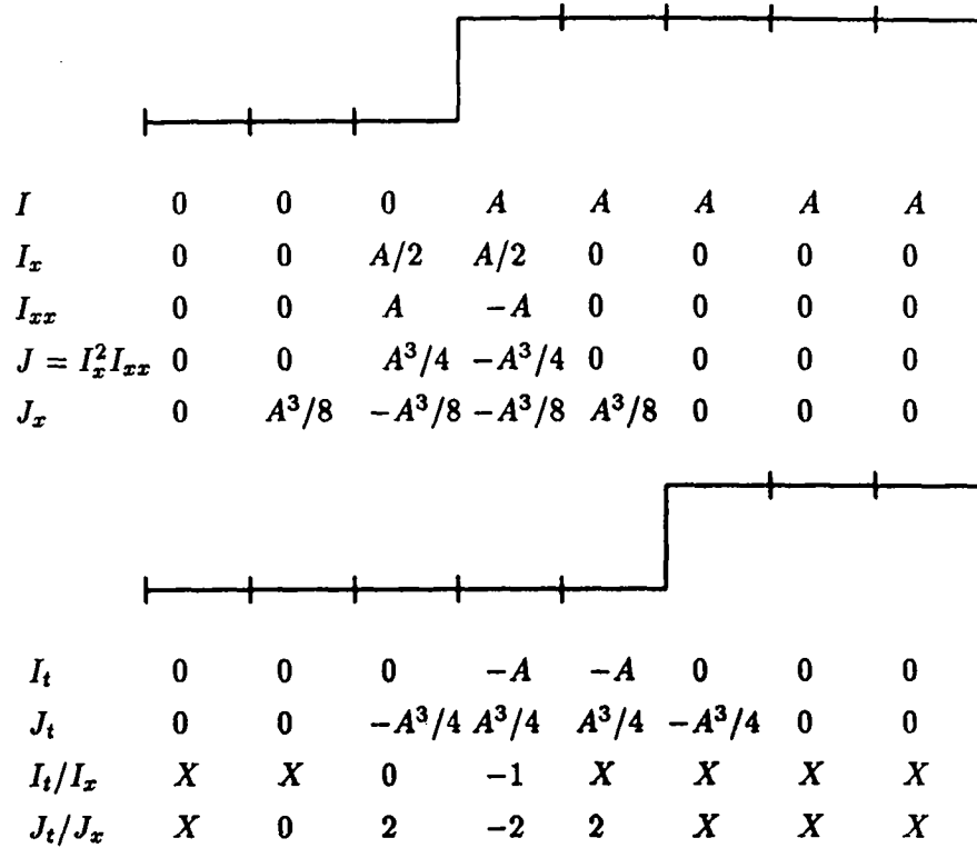
Figure 25: Showing derivatives computation of a 1D-edge
