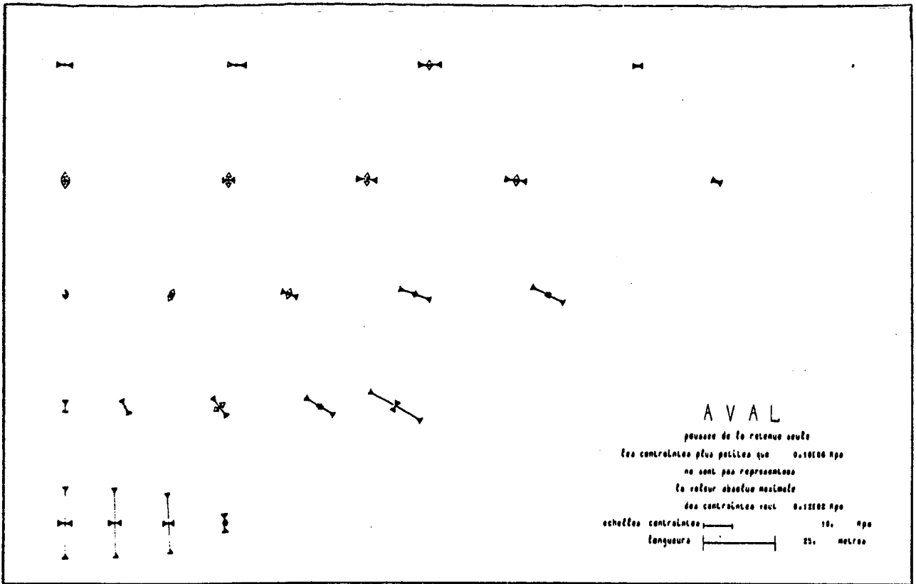
Fig. 6.1a : Stress distribution on downstream face (8 triangles, \nu=0.2 )
