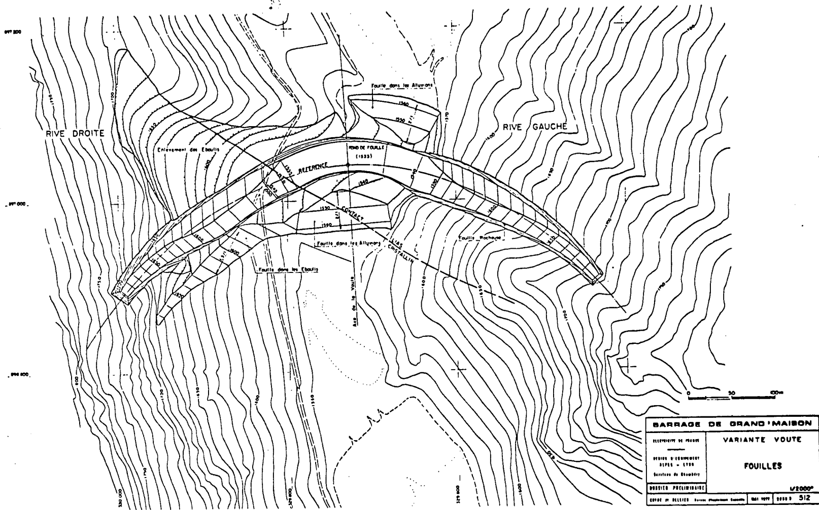
Figure 2.3 - Site plane of the dam (excavations)
