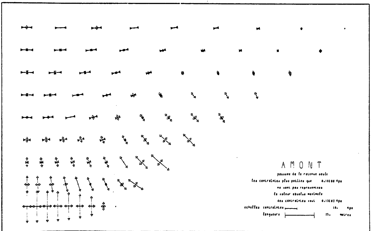
Fig. 6.1f : Stress distribution on upstream face (32 triangles, \nu = 0.2 )
