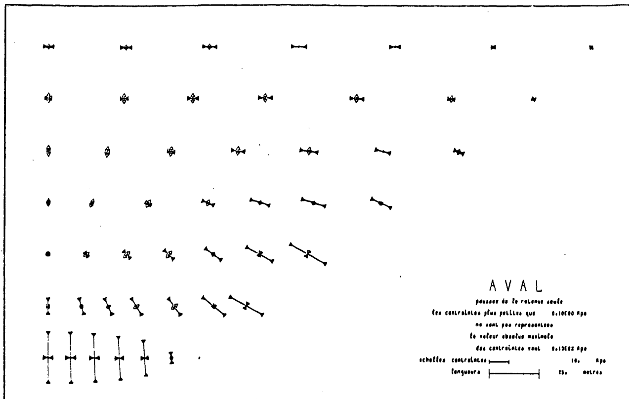
Fig. 6.1c : Stress distribution on downstream face (18 triangles, \nu = 0.2 )
