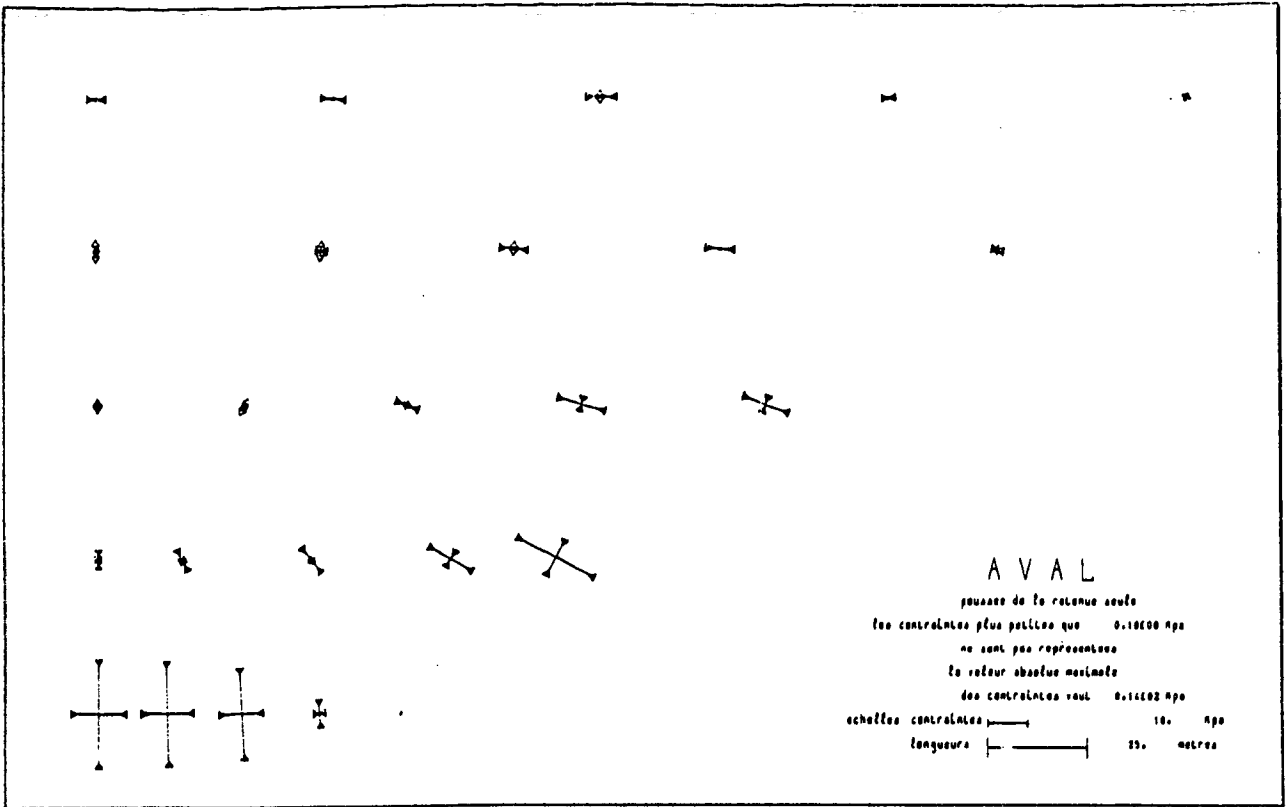
Fig. 6.2a : Stress distribution on downstream face ( 8 triangles, \nu = 0.495 )
