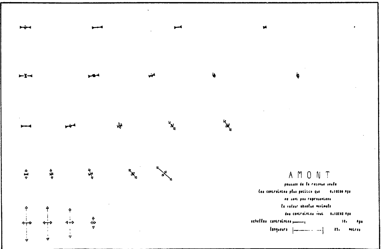
Fig. 6.1b : Stress distribution on upstream face (8 triangles, \nu = 0.2 )
