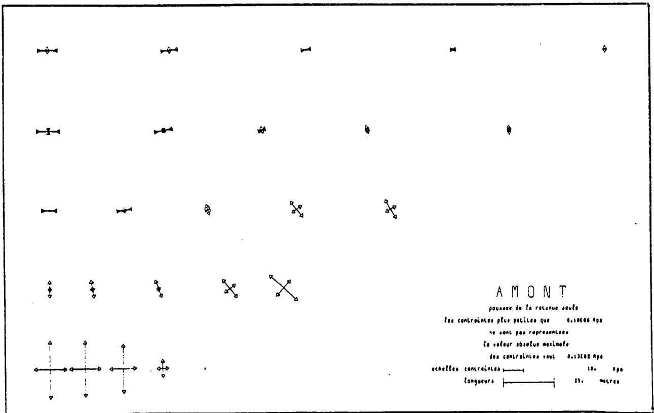
Fig. 6.2b : Stress distribution on upstream face ( 8 triangles, \nu = 0.495 )
