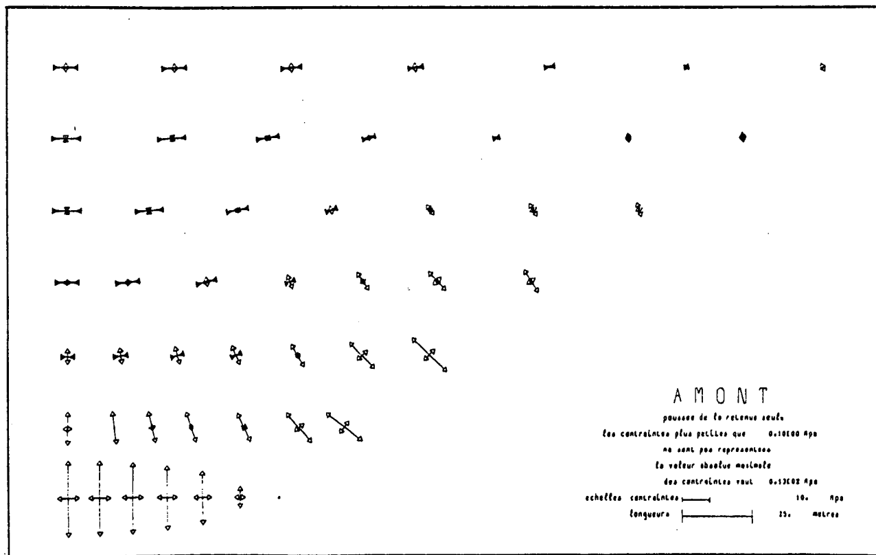
Fig. 6.1d : Stress distribution on upstream face (18 triangles, \nu = 0.2 )
