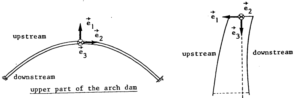
Figure 2.2 : the orthonormal reference system of the space G^3 .
