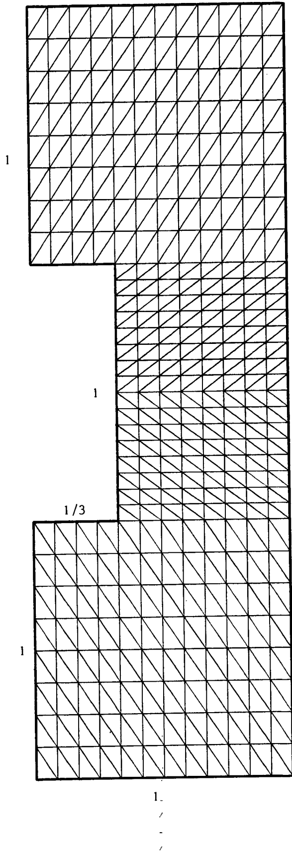
Fig. 1 - Triangulation : 640 triangles and 369 vertices.
