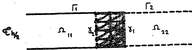
\mathcal{P}_1 - iso \mathcal{P}_2 VELOCITY GRID WITH OVERLAPPING
