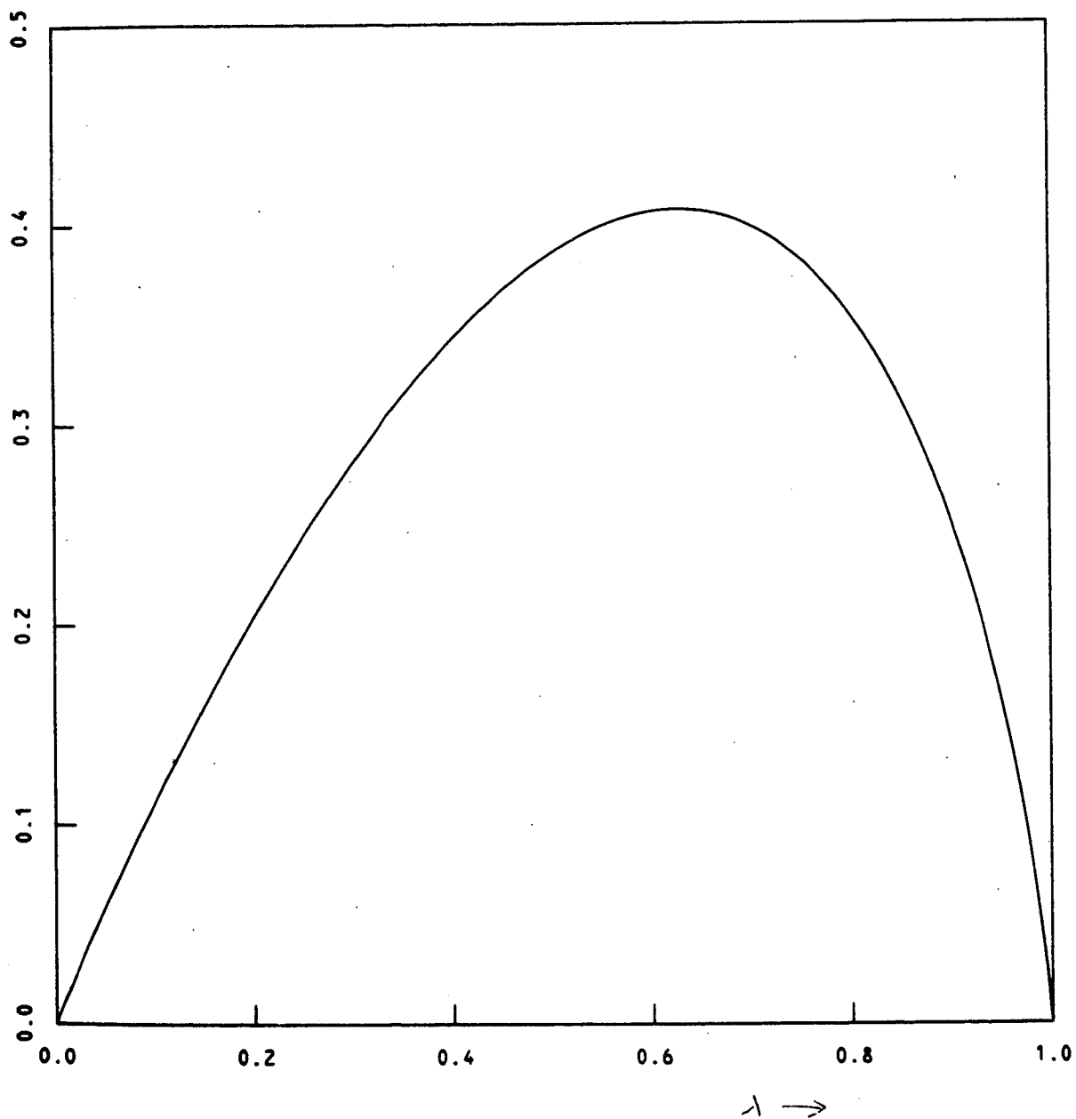
Fig. 2. The function f(\lambda) , which equals the limit of 2^{-h} \log B_{h,n} as h, n \rightarrow \infty with n \sim \lambda 2^h .
