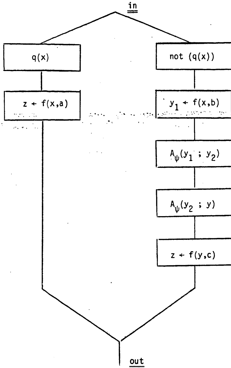
Fig.13 A_{\psi}(x; z)
