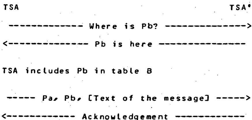
figure 3.7 : The complete distant transport protocol
