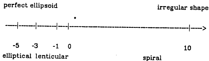
figure 1 The continuous labeling T
